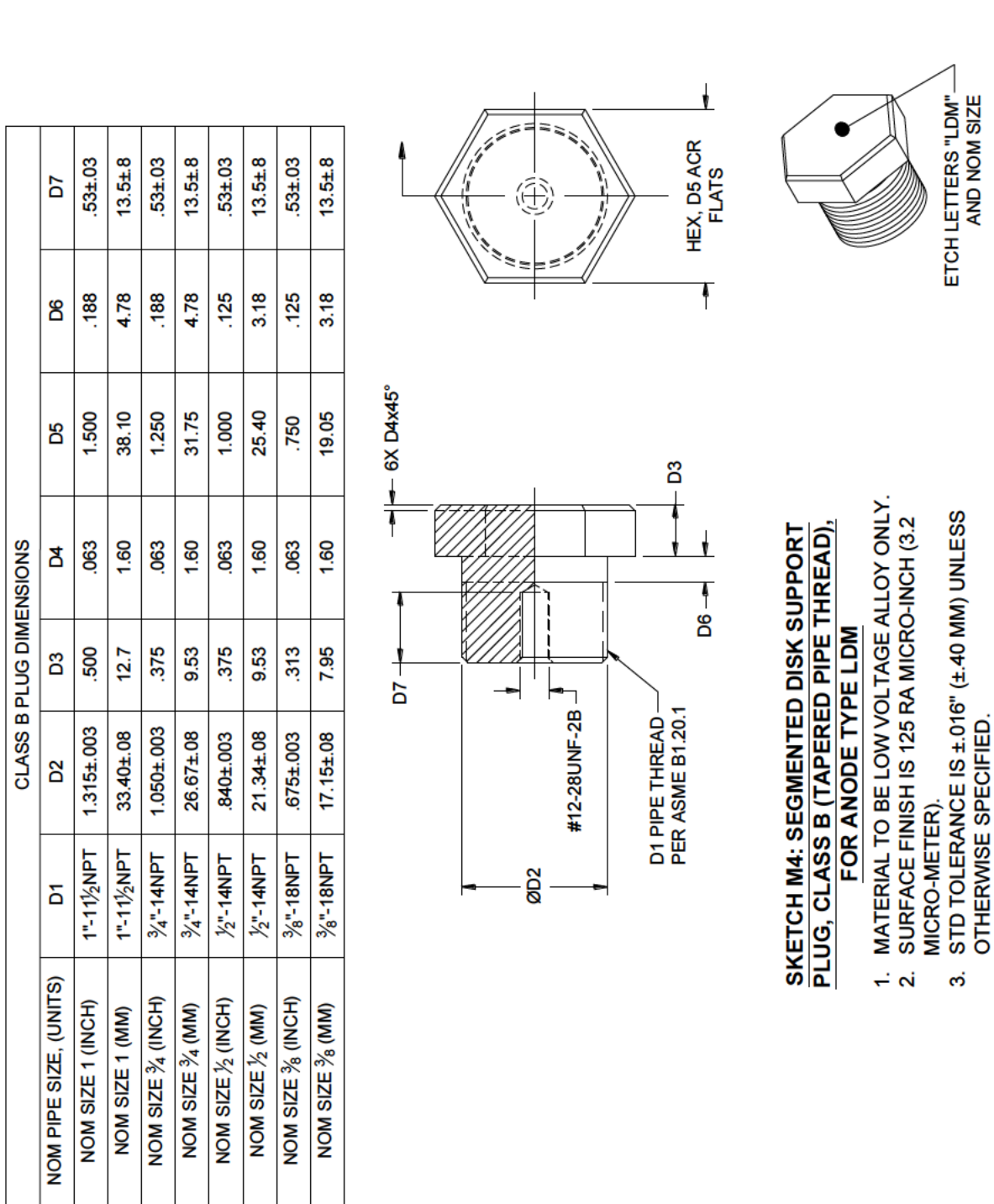
FIGURE A-47. Aluminum, segmented disk support plug, class B (tapered pipe thread) type LDM.
